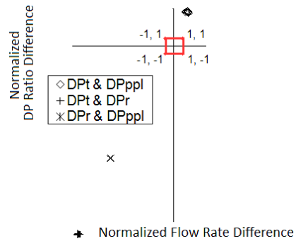
Fig 31. Rock trapped at orifice plate NDB plot.
