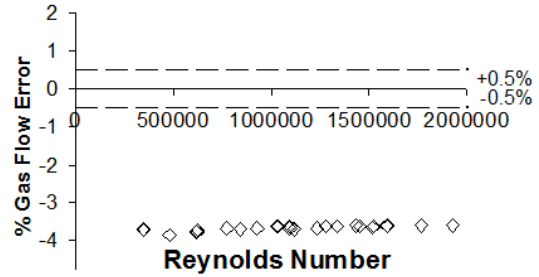
Fig 24. A heavily contaminated plate meter error.
