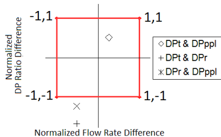
Fig 28. Light liquid load wet gas flow NDB plot.
